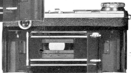
CONTAX Focal-plane Shutter partly open
